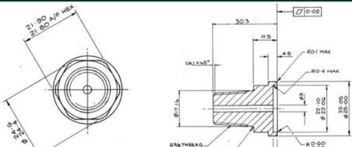
227-387-01 R38 Male (PT3/8) A-A3-3271$01
