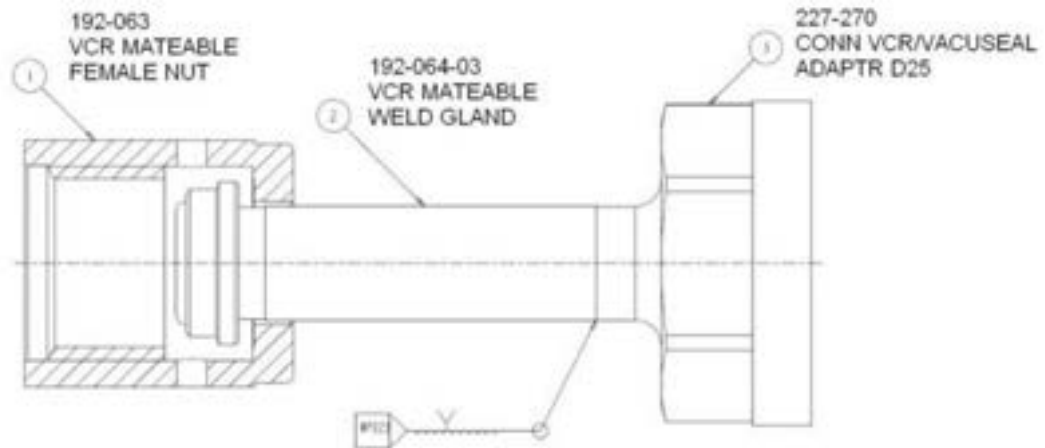
DA6831-1-01 VCR Female A-A3-6831$01A
