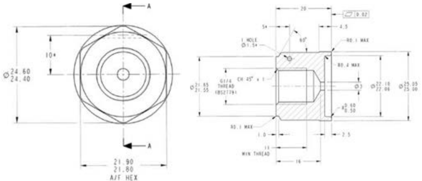
227-240 Conn G1/4 Female D25 316 Push A-A3-1709$02C
