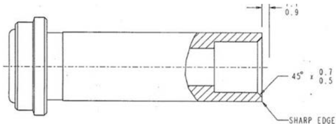
192-064-01 VCR Mateable Weld Gland A-A4-1504$03A
