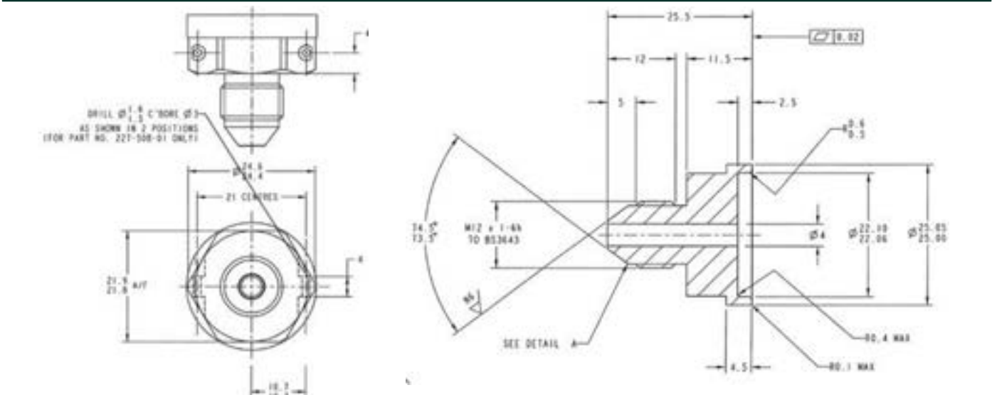
227-508-01 M12 X 1.0 74 0 External Cone A-A3-3617$01B
