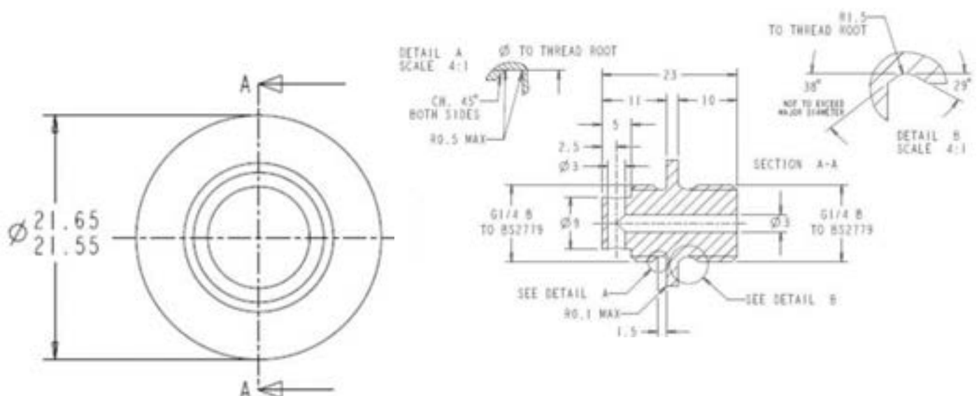
190-669-01 Adapter Core G1/4 Male to G1/4 Male A-A4-9055$01A
