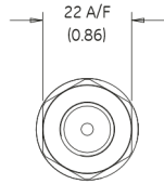
MALE PRESSURE CONNECTION
