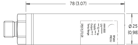
MEDIUM PRESSURE CONSTRUCTION
