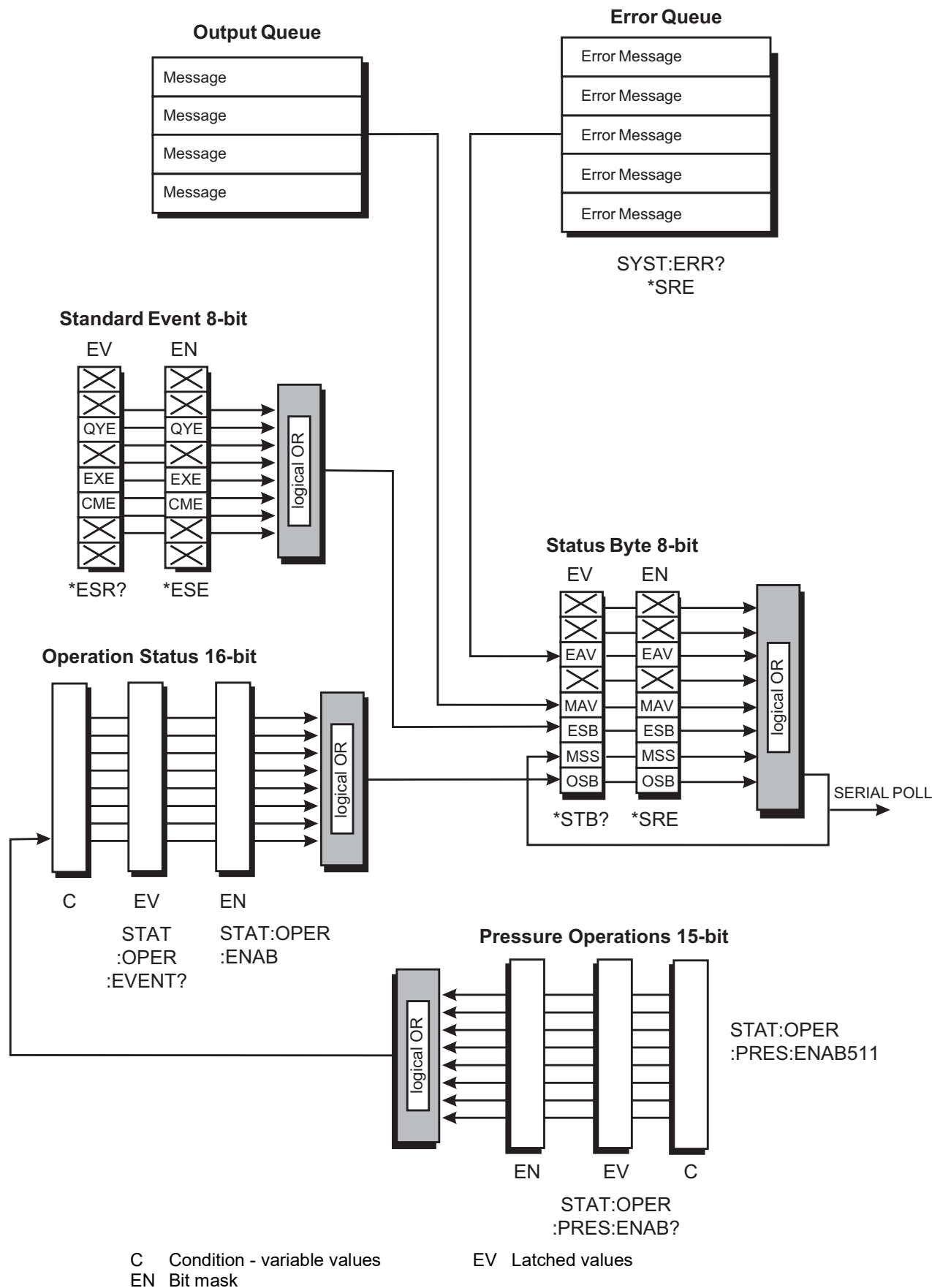
Figure 3-1: Status System
