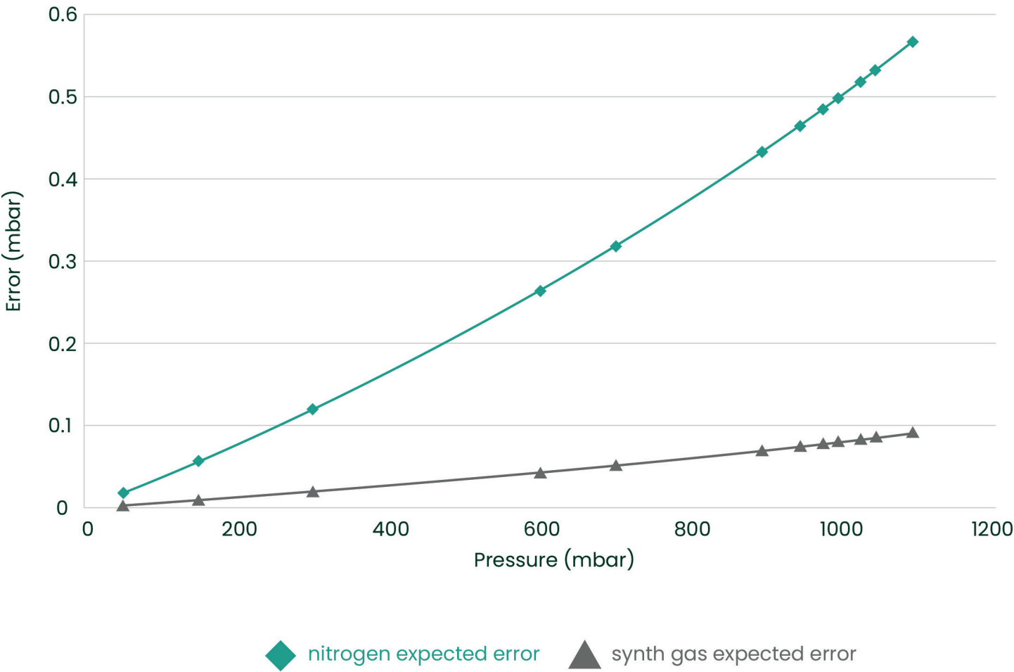
Figure 6: Density of gas impact on the measurement error
