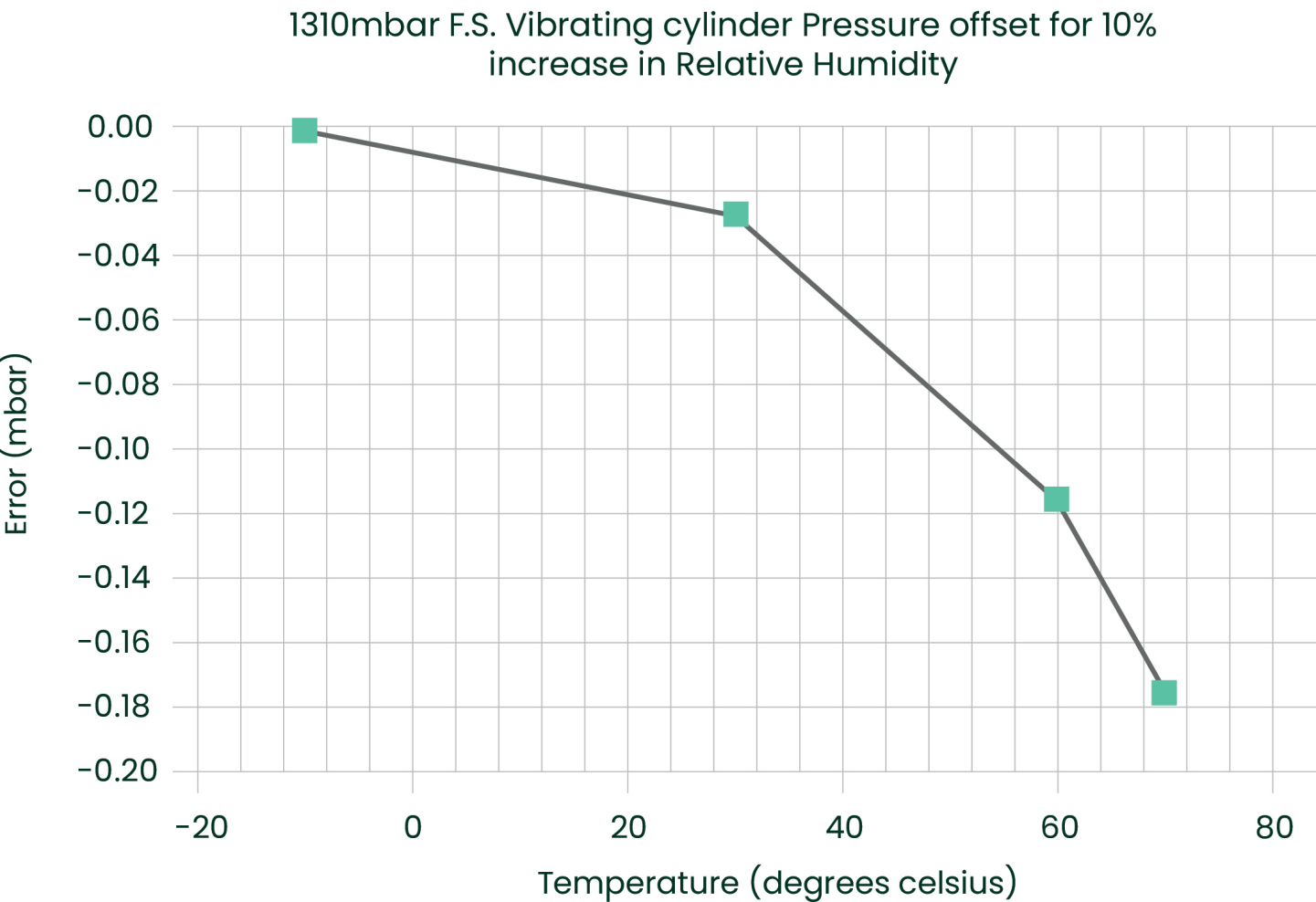
Figure 5: Pressure offset dependency relative to humidity
