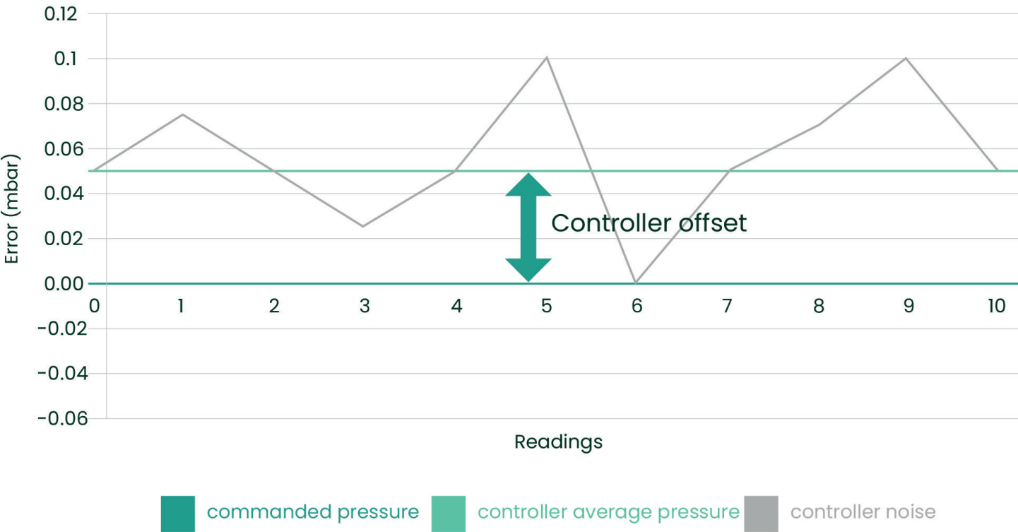
Controller offset and noise
