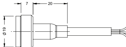
POLYURETHANE/RAYCHEM CABLE
