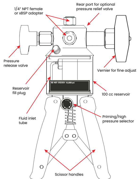
PV212-X components
